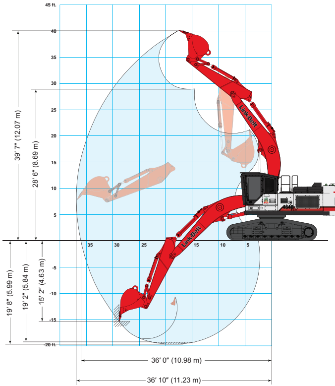
Boom Cylinders in High Lift Position
